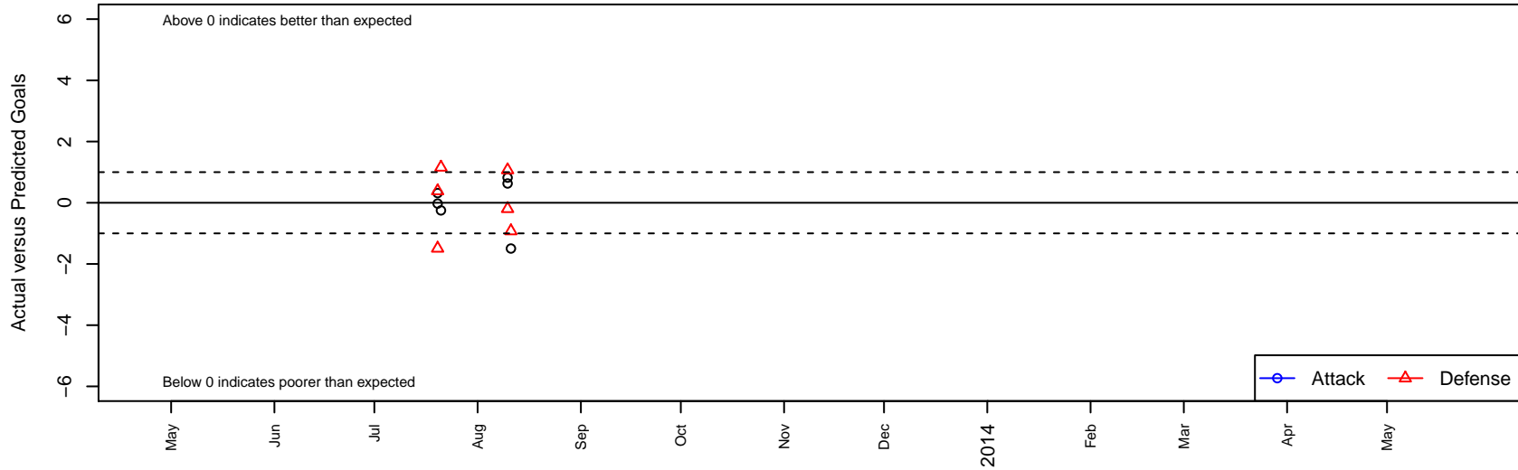
LA Premier FC G01 Dots are actual minus expected GF (blue circles) and GA (red triangles). Blue line is smoothed change in attack strength. Red is smoothed change in defense strength.
